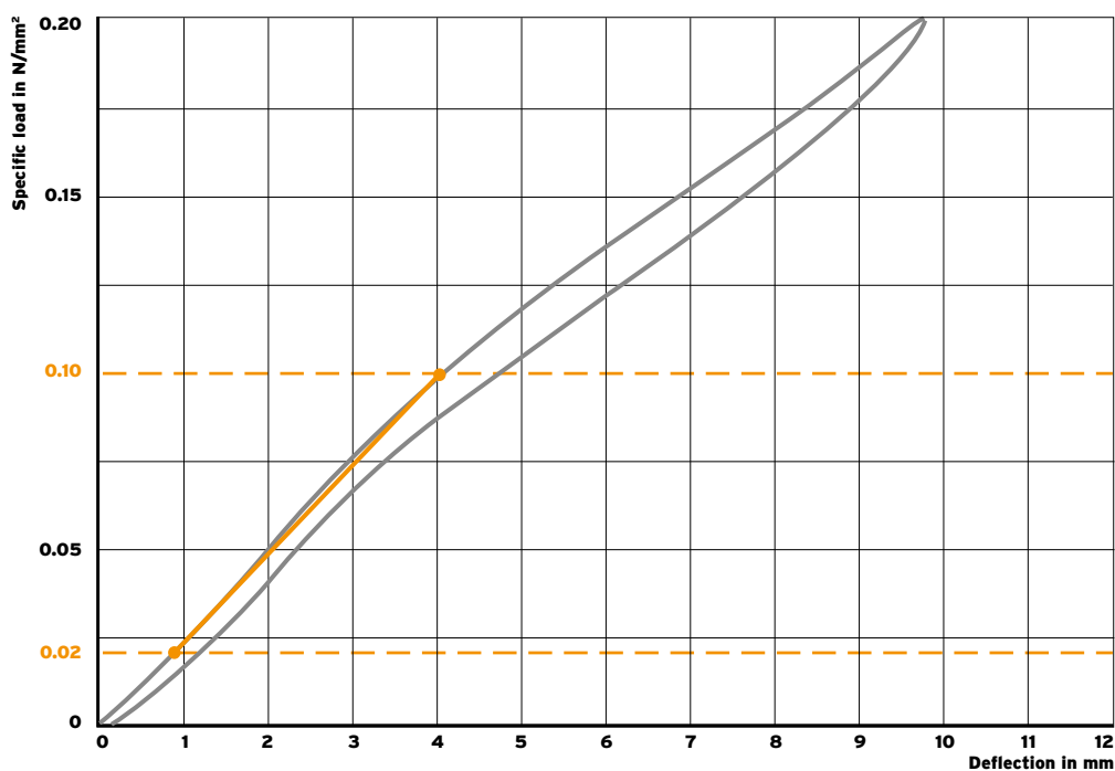
Spring load deflection curve for Syldyn® DN 335 under ballast mat
