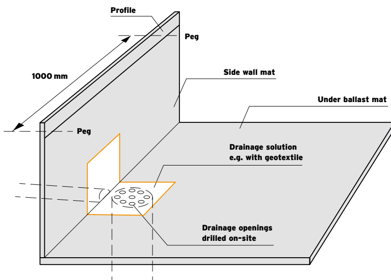
Drainage principle: Sylomer® and Sylodyn® under ballast mats
