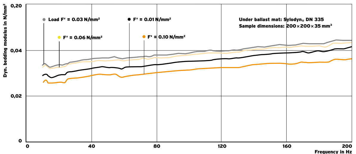
Load and frequency dependence of dynamic stiffness (from: Müller-BBM, Report No. 32242/12)
